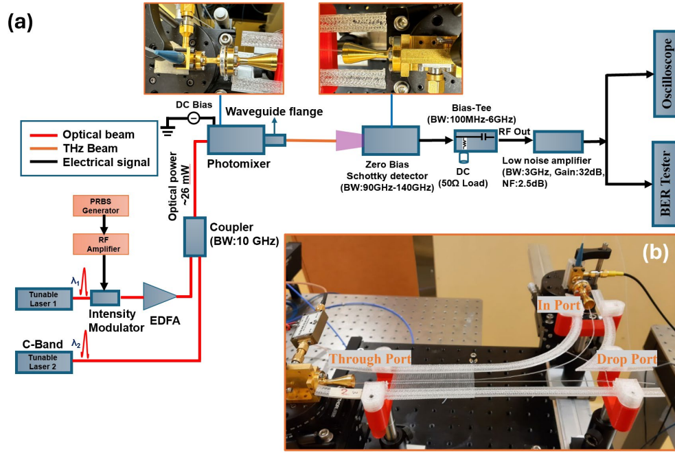
Fig. 3. (a) Schematic of the photonics-based THz communication system. (b) Photo of the measurement setup with a mounted device.
