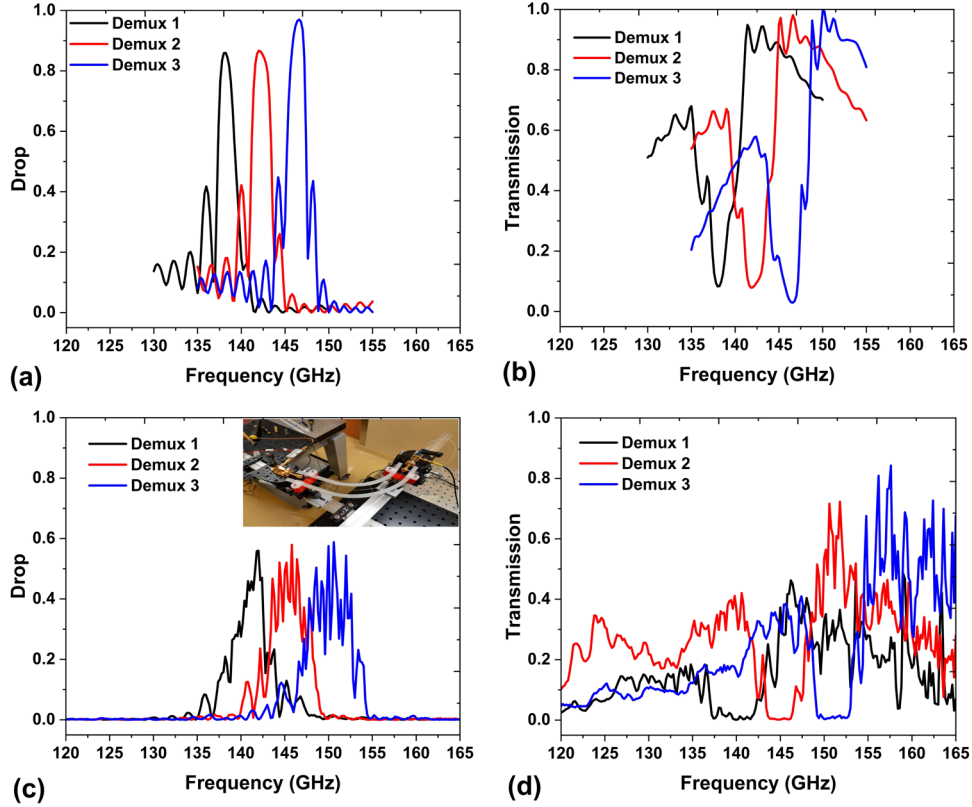
Fig. 4. (a) Drop and (b) Through spectra as predicted by numerical simulations. Relative (c) Drop and (d) Through coefficients when using transmission through a stand-alone bend as a reference. Insert: picture of a stand-alone waveguide bend.
