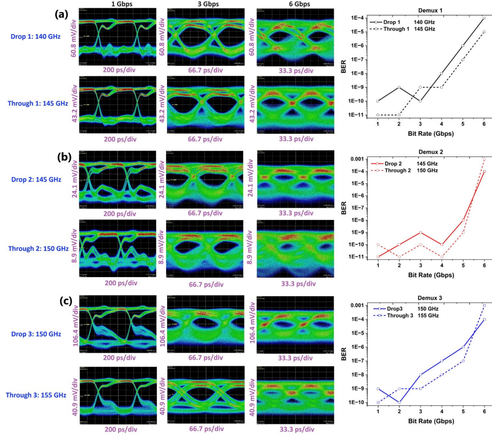
Fig. 5. Measured Bit Error Rate (BER) versus Bit Rate in the 1-6 Gbps range and the corresponding eye diagrams for 3 demultiplexers (a) Demux1 (b) Demux2, and (c) Demux3 at the Drop and Through ports.
