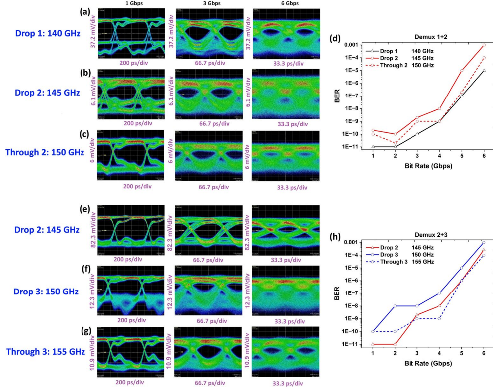
Figure 8. Measured Bit Error Rate versus Bit Rate and the corresponding eye diagrams for in-sequence Demux 1+2 at different bitrates (a) eye pattern at the Drop 1 port (b) eye pattern at the Drop 2 port (c) eye pattern at the Through 2 port (d) BER at the Drop 1, Drop 2, and Through 2 ports. Similar data is shown in panels (e)-(h) for Demux 2+3 and ports Drop 2, Drop 3, and Through 3 ports.
