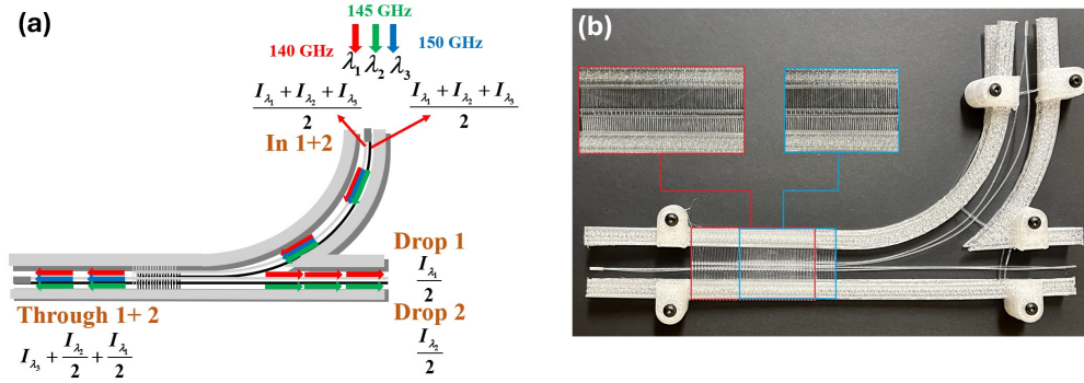
Fig. 9. (a) A schematic of the in-parallel demultiplexer (Demux 1||2). (b) A photo of the assembled device.
