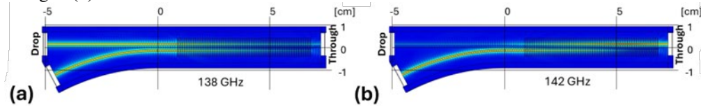
Fig. 2. Electric field amplitude distribution in the Demux1 operating at (a) Drop (138 GHz) and (b) Through (142 GHz) frequencies.
