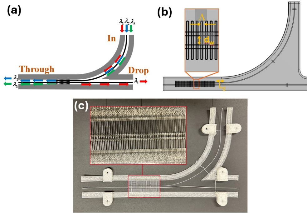
Fig. 1. (a) A schematic of a WDM demultiplexer (b) A typical computational cell used in numerical simulations. (c) A photo of a WDM demultiplexer. Inset: zoom of a grating section.
