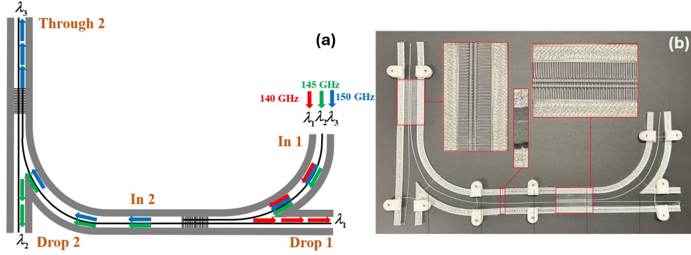
Fig. 6. (a) A schematic of the in-sequence demultiplexer (Demux 1+2). (b) A photo of the assembled device.
