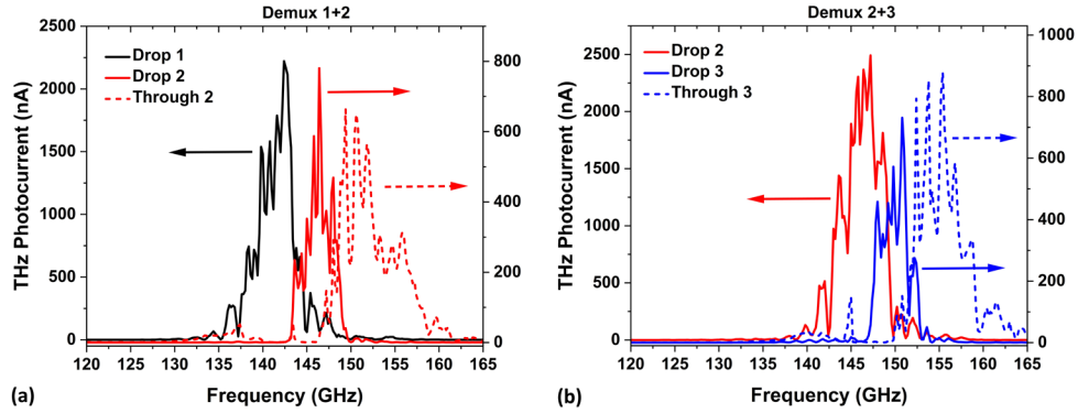
Fig. 7. (a) Experimental spectra of Drop 1, Drop 2, and Through 2 of the Demux 1+2. (b) Experimental spectra of Drop 2, Drop 3, and Through 3 of the Demux 2+3.
