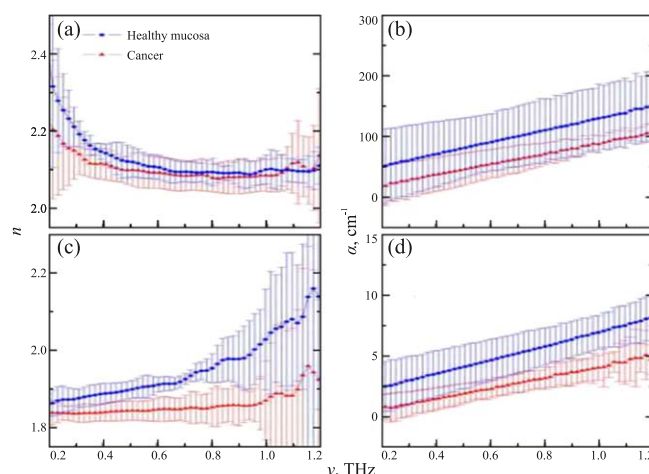
Figure 12. The THz refractive index n and absorption coefficient \alpha of normal mucosa and oral cancer ex vivo (mucoepidermoid carcinoma and squamous cell carcinoma (SCC)), averaged for six oral samples and measured at the temperatures of 20 °C (a), (b) and –20 °C (c), (d). Here, the dots represent the average values, while the error bars stand for the 95% confidence interval. Reprinted with permission from [271]. © The Optical Society of America.
