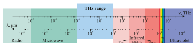
Figure 1. The THz range of the electromagnetic spectrum, where \nu and \lambda stand for the electromagnetic wave frequency and wavelength, respectively. Courtesy of K I Zaytsev.
