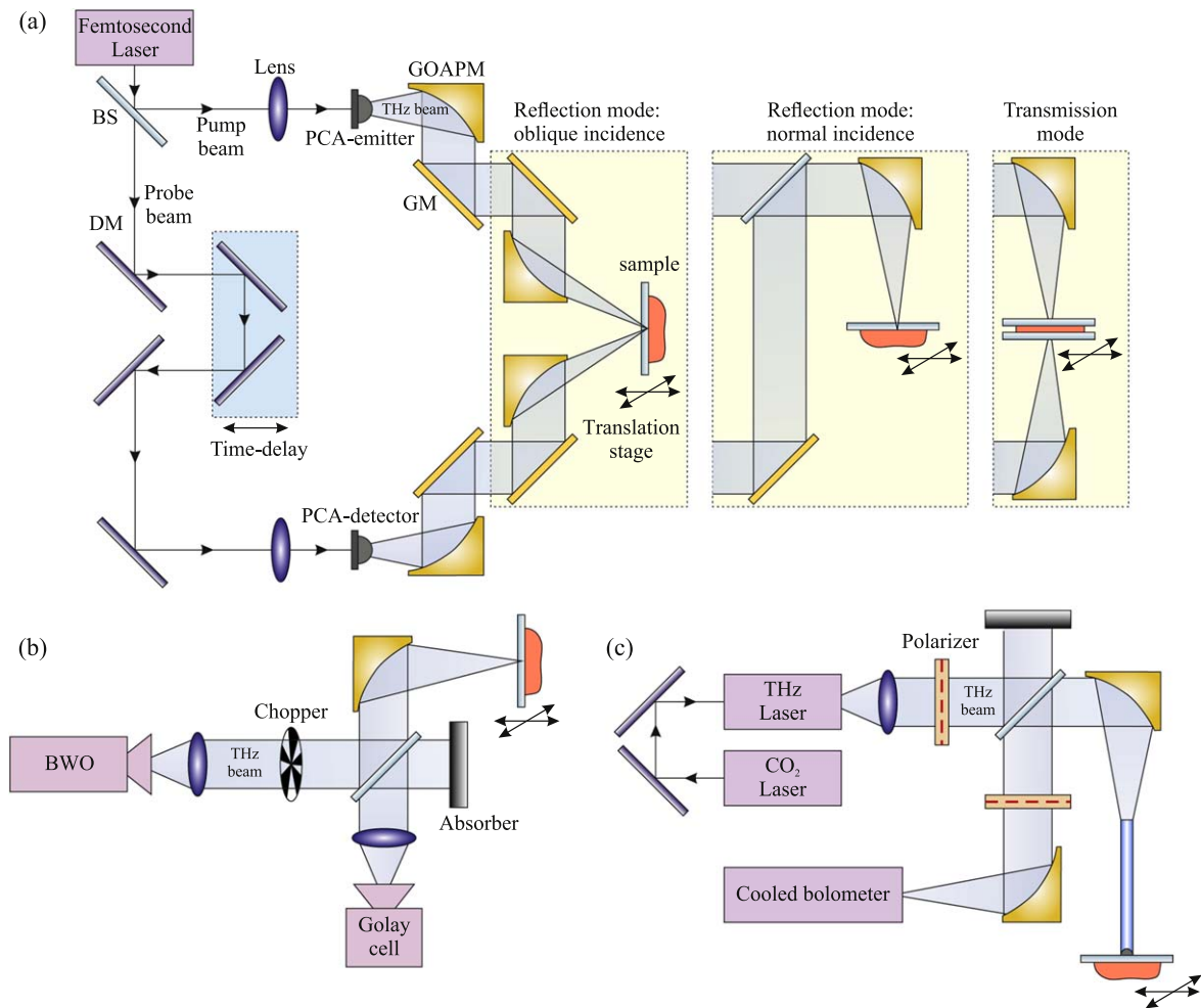
Figure 8. Common tissue measurement schemes in the THz range: (a) imaging and spectroscopy using TPS in reflection and transmission modes, (b) CW imaging and spectroscopy using BWO and the Golay cell, (c) a promising scheme of THz imaging system equipped by the waveguide, a CO 2 pumped THz gas laser and a cooled bolometer; (b), (c) are both in reflection mode and admit transmission mode as well. Here, BS stands for beam-splitter, GOAPM is the THz gold off-axis parabolic mirror, DM is the NIR dielectric mirror and GM is the THz gold mirror. Courtesy of I N Dolganova.
