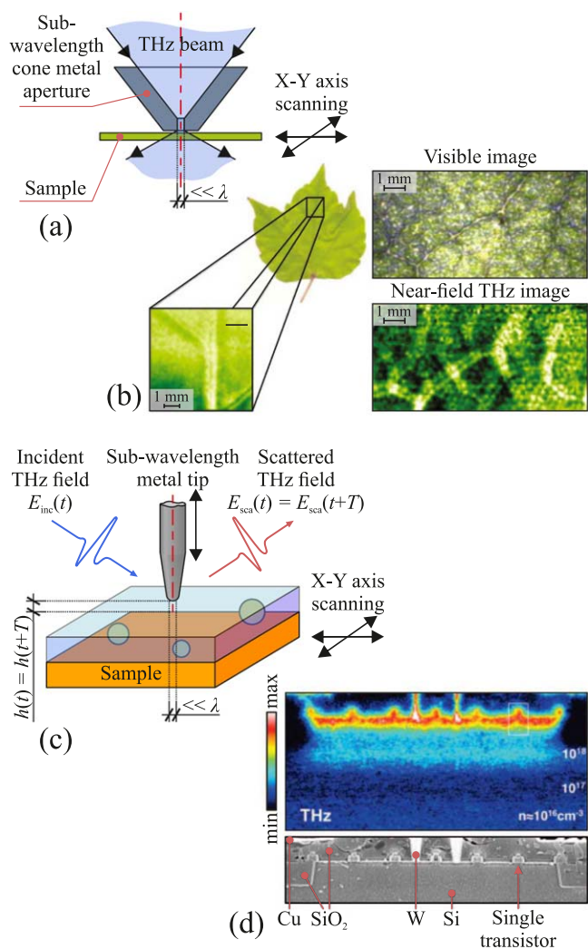
Figure 21. Representative examples of two distinct types of the THz near-field scanning-probe microscopy: (a), (b) a scheme of the 0.15\lambda -resolution THz microscope based on a cone metal aperture/diaphragm, as well as results of its application for the imaging of a leaf, respectively; (c), (d) a scheme of the 10^{-3}\lambda -resolution THz microscope based on a metal tip/cantilever, as well as results of its application for the imaging of a microelectronic device. (a), (b) Reprinted from [412], with the permission of AIP Publishing. (d) Reprinted with permission from [409]. Copyright 2008 American Chemical Society.
