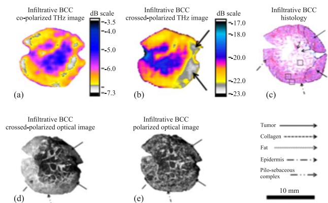
Figure 11. Reflection-mode polarization-sensitive THz imaging of tissue specimen ex vivo with infiltrative BCC: (a) a co-polarized THz image; (b) a cross-polarized THz image; (c) a H&E-stained histology of the 5-mm thick frozen tissue section; (d) a cross-polarized optical image; (e) a co-polarized optical image. [110] John Wiley & Sons. Copyright © 2014 WILEY-VCH Verlag GmbH & Co. KGaA, Weinheim.
