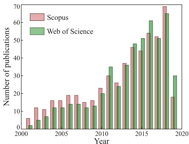
Figure 2. The annual number of publications (from 2000 to 2019) related to the terahertz diagnosis of malignancies, retrieved from the query ('terahertz' or 'THz') and ('malignancy' or 'cancer' or 'tumor') from the Scopus and Web of Science databases; search request dated May 6, 2019. Courtesy of A A Gavdush and K I Zaytsev.
