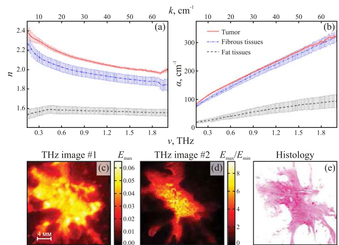
Figure 15. The reflection-mode TPS and TPI of human breast tumors ex vivo : (a), (b) the mean refractive index n and absorption coefficient \alpha of the tumor, fibrous and fat tissues, averaged within several specimens of the breast tissues, where the error bars represent a 95% confidential interval of measurements; (c)–(e) TPI images based on the maximal amplitude of the THz pulse \max_t[E(t)] and the normalized amplitude \max_t[E(t)]/\min_t[E(t)] , as well as results of histology. The ductal and lobular carcinomas of the breast were studied by the authors. Reprinted with permission from [54]. © The Optical Society of America.
