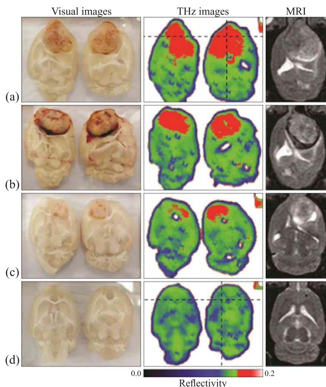
Figure 16. A comparison of visual, THz and MR images of freshly excised whole rat brain tissues with (a)–(c) and without (d) tumors. The dimensions of the THz images are 4 \times 3 \text{ cm}^2 , while the scanning resolution is 250 \mu\text{m} . An orthotopic glioma model from rats with clear tumor margins is used. Reprinted with permission from [55]. © The Optical Society of America.
