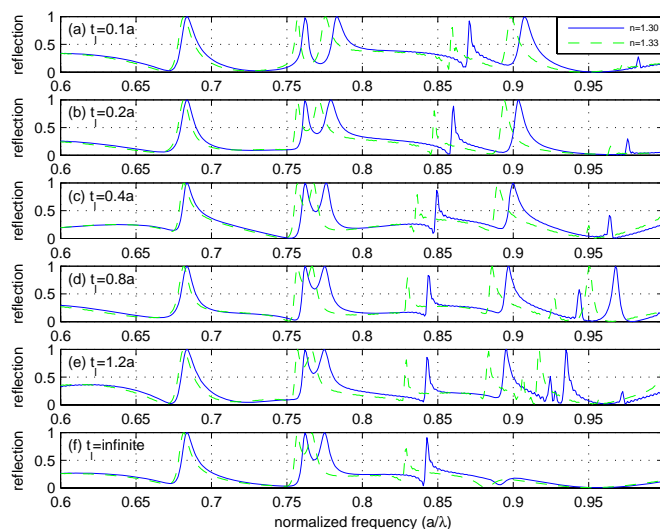
Fig. 6. Reflection spectra of six PhC slabs with different analyte thicknesses t_l : 0.1a , 0.2a , 0.4a , 0.8a , 1.2a , \infty .
