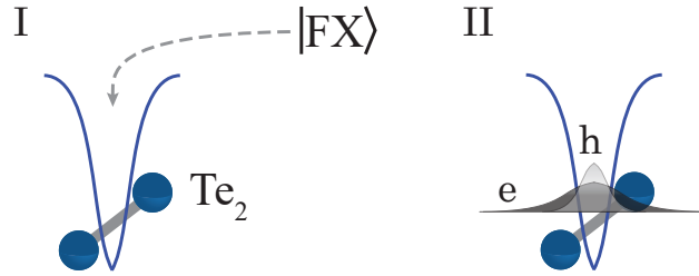
Figure 4.6 One-step binding mechanism of a FX to a \text{Te}_2 molecule. After its photo-generation, the FX diffuses in the lattice and falls into the narrow potential well created by the molecule (I), creating a bound exciton (II).
