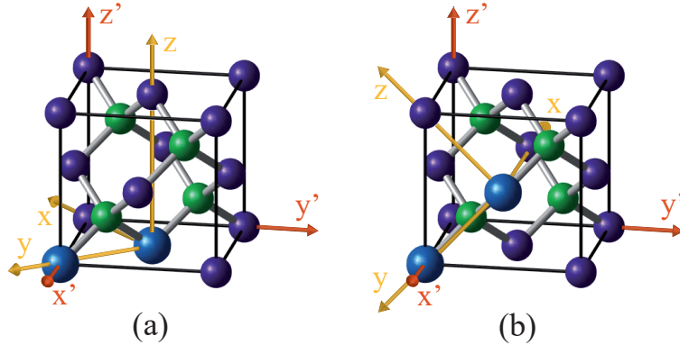
Figure 1.2 \text{ZnSe} lattice with (a) in-plane and (b) out-of-plane \text{Te}_2 molecules. Red axes are lab coordinates, while yellow ones are that of the defect. Green, purple and blue spheres are respectively Zn, Se and Te atoms.
