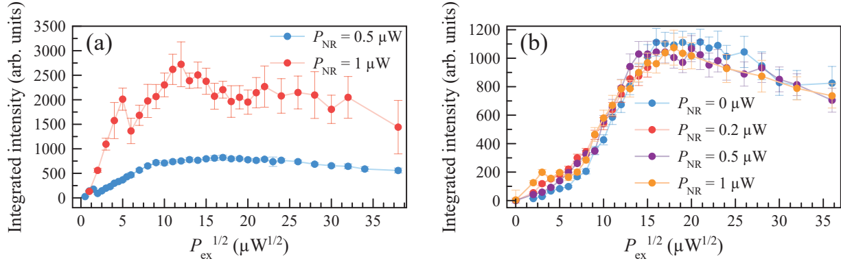
Figure 6.19 Resonant PL I_{em} as a function of resonant P_{ex}^{1/2} for different P_{NR} , showing a saturation of I_{em} . (a) Emitter for which P_{NR} dramatically influenced I_{em} . (b) Emitter for which P_{NR} did not impact the emission curve.
