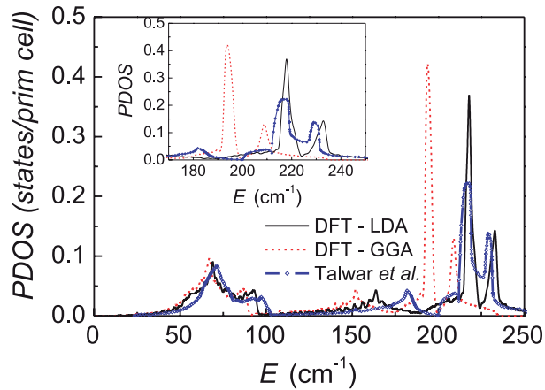
Figure 5.27 Calculated phonon density of states (PDOS) for ZnSe. The first local maximum happens at \sim 8.5\text{--}9.1 meV. Reprinted with permission from Ref. [197]. Copyright (2012) by the American Physical Society.
