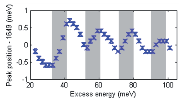
Figure 5.25 E_{em} oscillation of the FX emission line in monolayer \text{MoSe}_2 as a function of excess energy E_{ex} - E_{FX} . The minimum displacement happens when I_{em} is maximum (grey regions). Adapted with permission from the supplementary material of Ref. [195], Chow et al. , © The Authors 2017, Creative Commons Attribution 4.0 International License, https://creativecommons.org/licenses/by/4.0/ .
