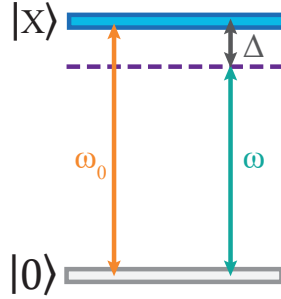
Figure 2.11 Two-level system formed of the n = 1 energy level of an exciton and its ground state (absence of an exciton). \omega_0 is the resonance frequency of the system, \omega , that of the driving electric field, and \Delta = \omega - \omega_0 is the detuning between the transition and the field.
