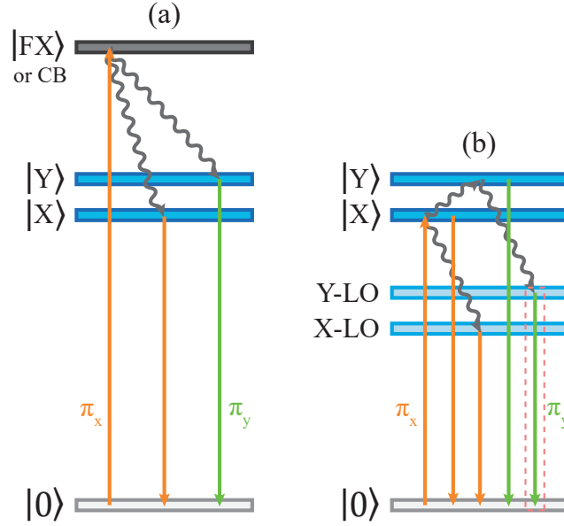
Figure 3.4 Energy levels, transitions and polarizations relevant the two experiments, allowing for spectral and polarization filtering. Excitation of the bandgap or the FX (a) leads to population of both X and Y regardless of the polarization. Resonant excitation of the X level (b) transfers population to Y , X -LO and Y -LO through non-radiative transfer mechanisms. The detected transition, Y -LO for the case illustrated, is indicated with a pink dashed box.
